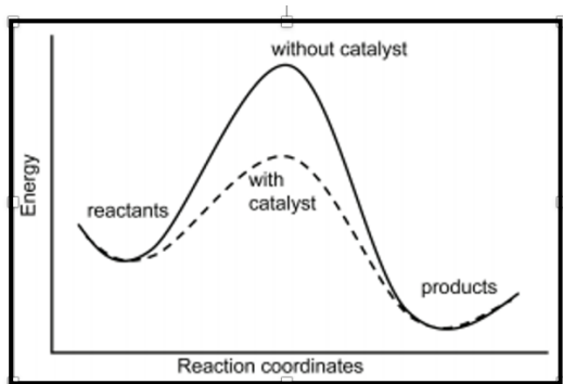
Figure 1. Chemical reaction without and with a catalyst.
